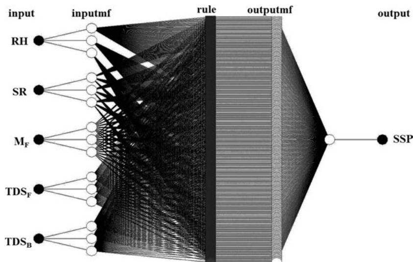
Figure 3 | ANFIS model structure used in this study ( RH : relative humidity; SR : solar radiation; M F : feed flow rate; TDS F : total dissolved solids of feed; TDS B : total dissolved solids of brine; SSP : solar still productivity).
